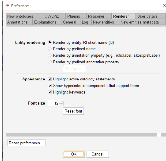
Figure 4.2 Renderer tab
